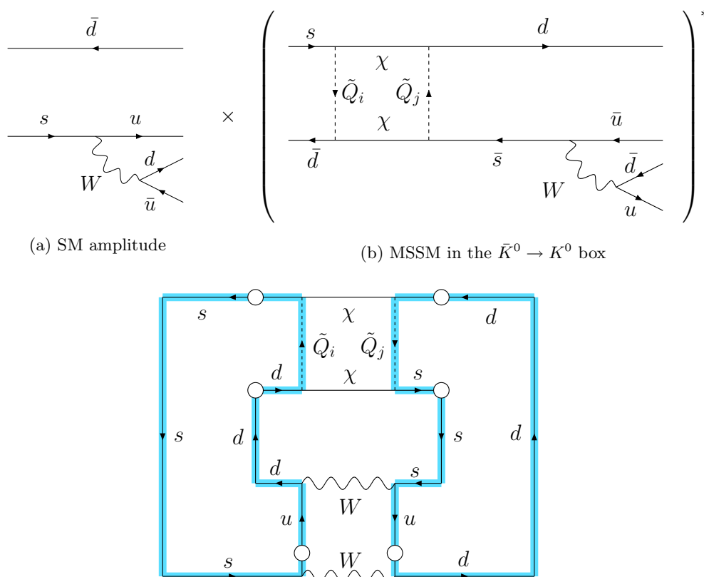
Figure 2: CP violating contribution in K^0 \rightarrow \pi\pi .
