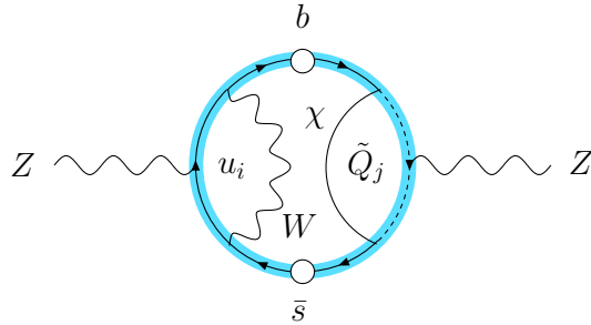
Figure 1: Interference term contributing to \Gamma(Z \rightarrow b\bar{s}) - \Gamma(Z \rightarrow \bar{b}s) .
